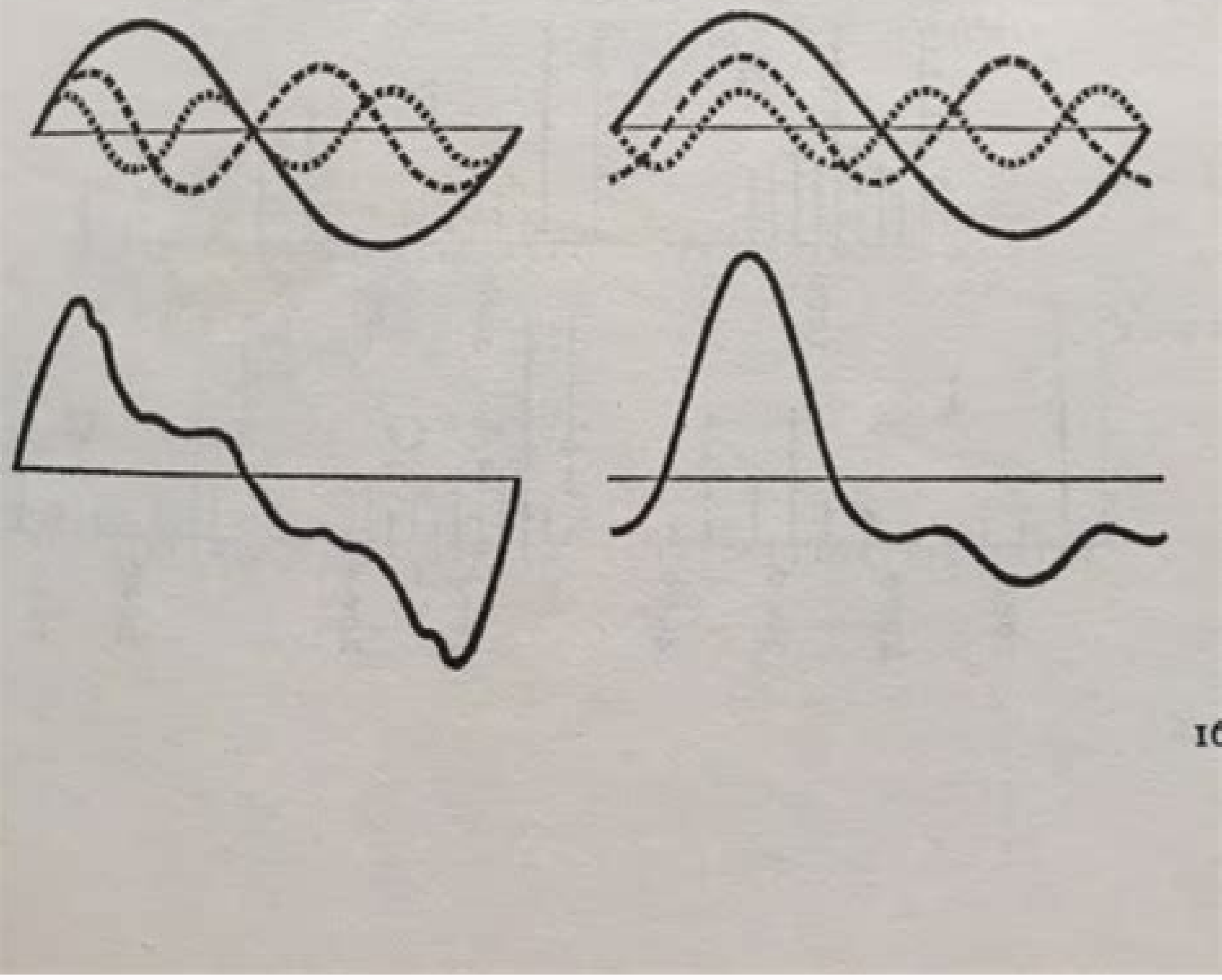
Figure 68. Two sound waves made up of the same fundamental and two harmonics, but in different phase relationship.
